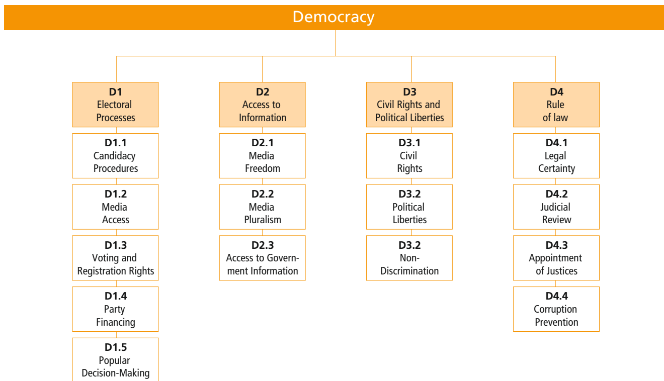
Figure 2: Democracy
