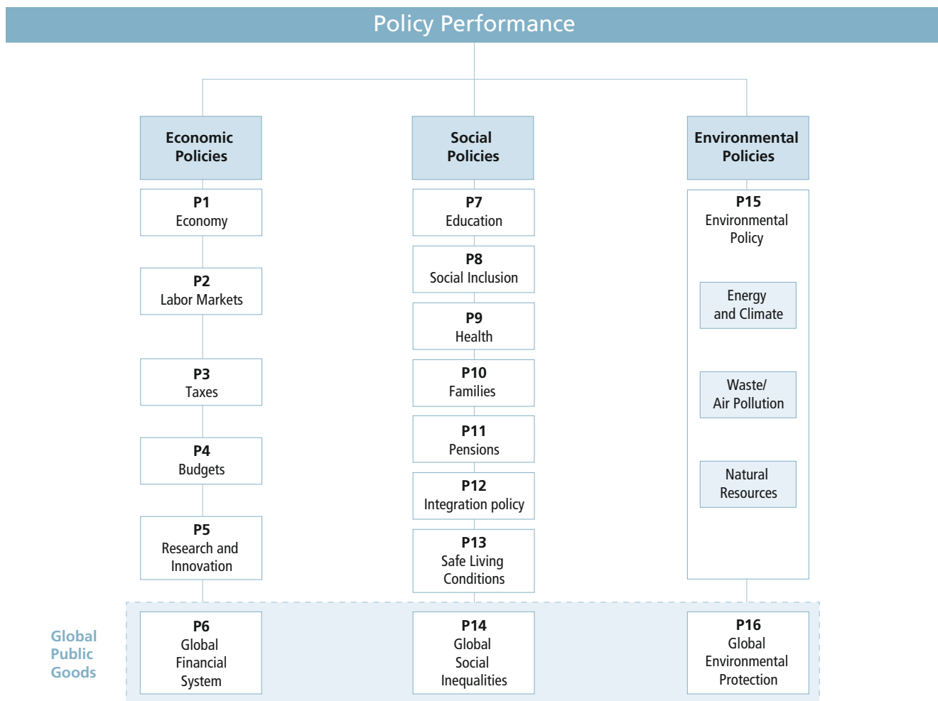
Figure 1: Policy Performance
